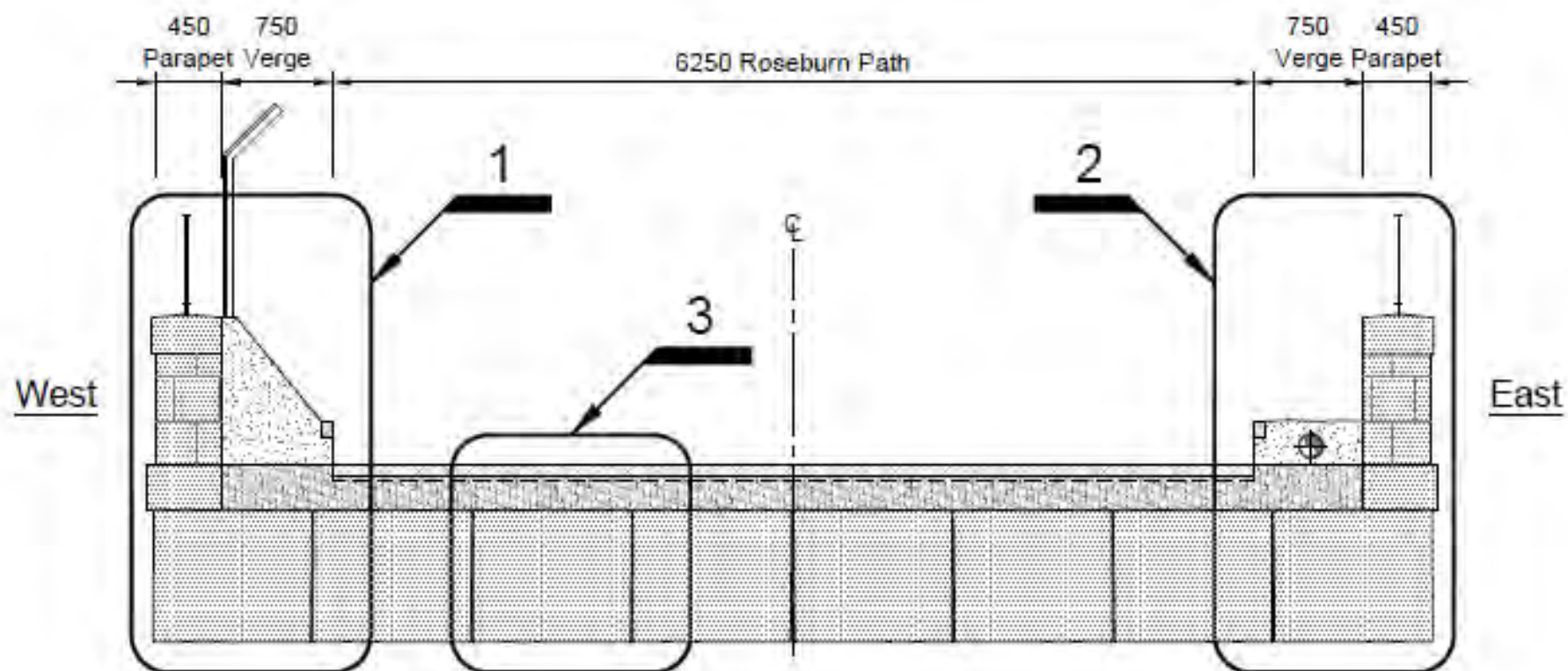
Typical Cross Section @ Arch Crown
